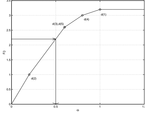
Figure 2. An illustration of the solution of the QP problem using the inverse of F(\theta) for \bar{D} = (1.0, 0.2, 0.6, 0.8, 0.6) . The optimal value is the solution for the equation F(\theta) = 2.2 which is 0.5.
