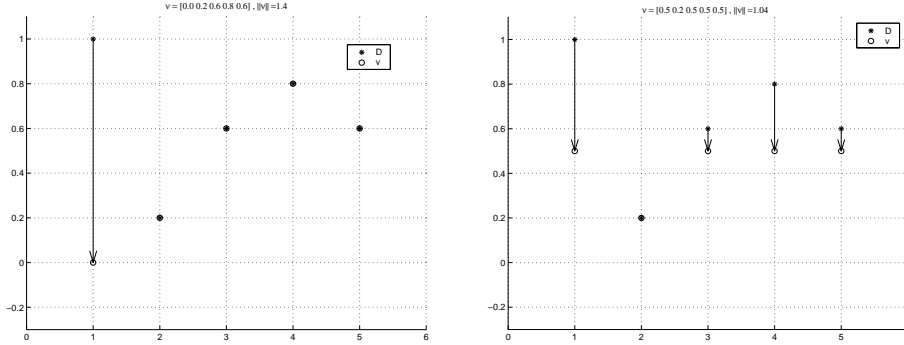
Figure 1. An illustration of two feasible points for the reduced optimization problem with \bar{D} = (1.0, 0.2, 0.6, 0.8, 0.6) . The x-axis is the index of the point, and the y-axis denotes the values \bar{\nu} . The right plot has a smaller variance hence it achieves a better value for \mathcal{Q} .
