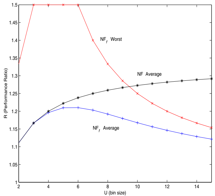
Fig. 2. Expected and worst case performance ratio of NF and NF_f with r = 1 , for values of U \leq 15 .
