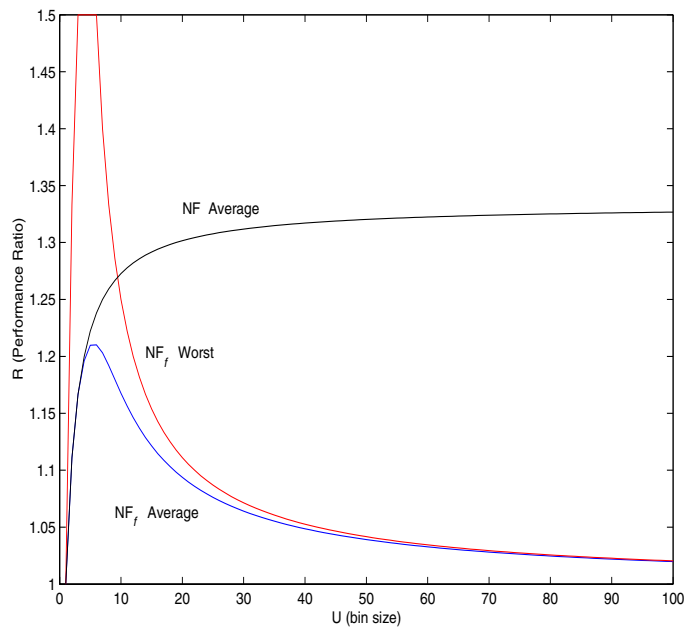
Fig. 1. Expected and worst case performance ratio of NF and NF_f with r = 1 .
