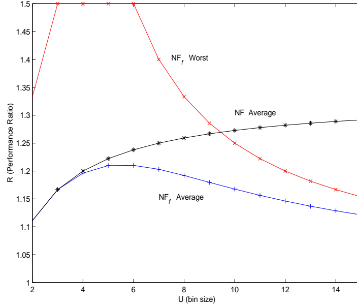
Fig. 2: Expected and worst case performance ratio of the NF_f and NF algorithms for values of U \leq 15 .
