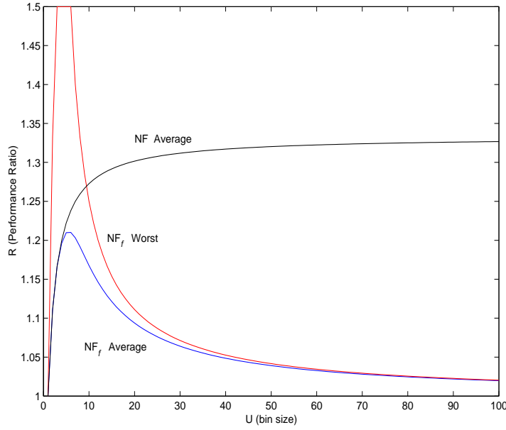
Fig. 1: Expected and worst case performance ratio of the NF_f and NF algorithms.
