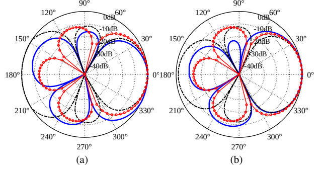
Fig. 2: Beampatterns for the second-order asymmetric hypercardioid CDMA's (blue solid line) and its symmetric version (black dashed line). The red circles line is the second-order unconstrained symmetric hypercardioid [6]. (a) \theta_1 = 60^\circ , \theta_2 = 110^\circ . (b) \theta_1 = 120^\circ , \theta_2 = 295^\circ .
