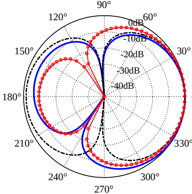
Fig. 4: A first-order asymmetric hypercardioid beampattern (blue solid line) obtained by (28) and a symmetric beampattern (black dashed line) obtained by imposing symmetry, for the case of M = 3 sensors, and desired null at \theta_1 = 95^\circ . The red circles line is the first-order unconstrained hypercardioid [6].
