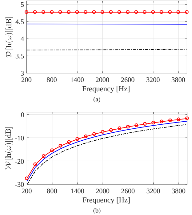
Fig. 6: DF (a) and WNG (b) vs. frequency for the first-order asymmetric hypercardioid (blue solid line), the optimal unconstrained symmetric hypercardioid (red circles line), and the symmetric design (black dashed line) with M = 3 sensors.
