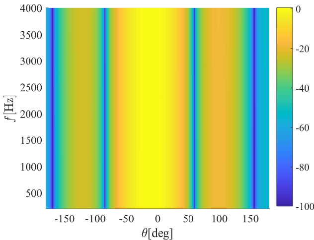
Fig. 10: A top view of the beam pattern versus frequency and \theta for the asymmetric second-order hypercardioid CDMA implemented in Section VI-D.
