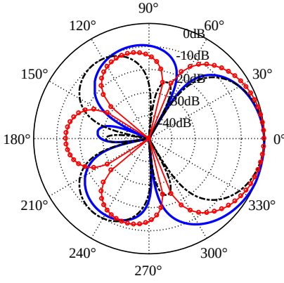
Fig. 7: An asymmetric second-order hypercardioid beampattern (blue solid line) obtained by (28) for the case of three imposed nulls and M = 5 microphones. Also presented the corresponding third-order symmetric beampattern (black dashed line) for the case of M = 7 sensors, and desired nulls at \theta_1 = 60^\circ , \theta_2 = 190^\circ , and \theta_3 = 275^\circ . The red circles line is the second-order unconstrained hypercardioid [6].
