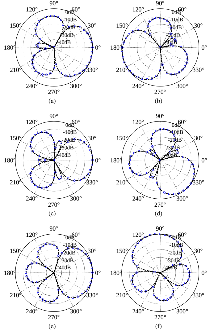
Fig. 8: Beampatterns of the second-order asymmetric hypercardioid CDMA with M = 5 sensors and three imposed nulls for different steering angles and frequencies: (a) \theta_s = 0^\circ , f = 800 Hz, (b) \theta_s = 215^\circ , f = 1800 Hz. Beampatterns of the corresponding third-order symmetric design with M = 7 sensors: (c) \theta_s = 0^\circ , f = 200 Hz, (d) \theta_s = 315^\circ , f = 1900 Hz. Beampatterns of the second-order unconstrained symmetric hypercardioid: (e) \theta_s = 0^\circ , f = 1300 Hz, (f) \theta_s = 100^\circ , f = 3500 Hz. The black dashed line is the designed beampattern (65), while the blue circles line is the analytical beampattern (28).
