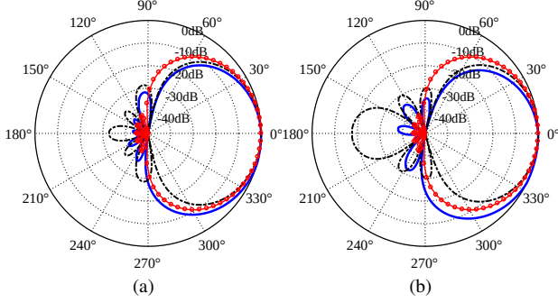
Fig. 3: Beampatterns for the third-order asymmetric supercardioid CDMA (blue solid line) and its symmetric version (black dashed line). The red circles line is the third-order unconstrained symmetric supercardioid [6]. (a) \theta_1 = 80^\circ , \theta_2 = 120^\circ , \theta_3 = 155^\circ . (b) \theta_1 = 75^\circ , \theta_2 = 105^\circ , \theta_3 = 220^\circ .
