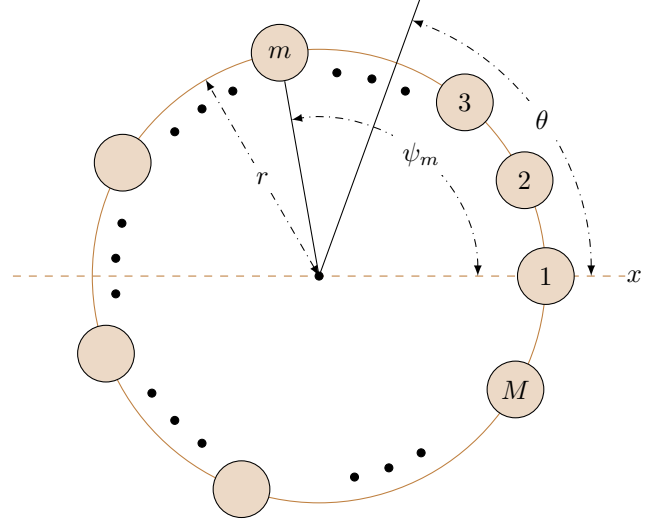
Fig. 1: Illustration of a uniform circular microphone array in the Cartesian coordinate system.
