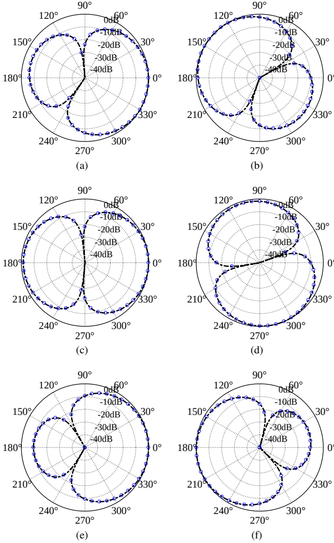
Fig. 5: Beampatterns of the first-order asymmetric hypercardioid using CDMA's with M = 3 sensors for different steering angles and frequencies: (a) \theta_s = 0^\circ , f = 600 Hz, (b) \theta_s = 155^\circ , f = 2400 Hz. Beampatterns of the corresponding first-order symmetric design: (c) \theta_s = 0^\circ , f = 1000 Hz, (d) \theta_s = 285^\circ , f = 3200 Hz. Beampatterns of the first-order unconstrained symmetric hypercardioid: (e) \theta_s = 0^\circ , f = 900 Hz, (f) \theta_s = 195^\circ , f = 2100 Hz. The black dashed line is the designed beampattern (65), while the blue circles line is the analytical beampattern (28).
