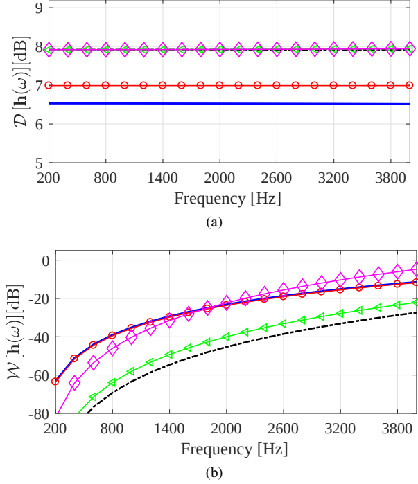
Fig. 9: DF (a) and WNG (b) vs. frequency for the second-order asymmetric hypercardioid (blue solid line), the second-order unconstrained symmetric hypercardioid (red circles line) with M = 5 sensors, and the third-order symmetric design (black dashed line) with M = 7 sensors. Also presented the third-order symmetric design (magenta diamonds line) with M = 15 sensors and larger array (element spacing, \delta = 0.65 cm), and the third-order symmetric design (green triangles line) with M = 20 sensors and the same size of original array ( r = 0.75 cm).
