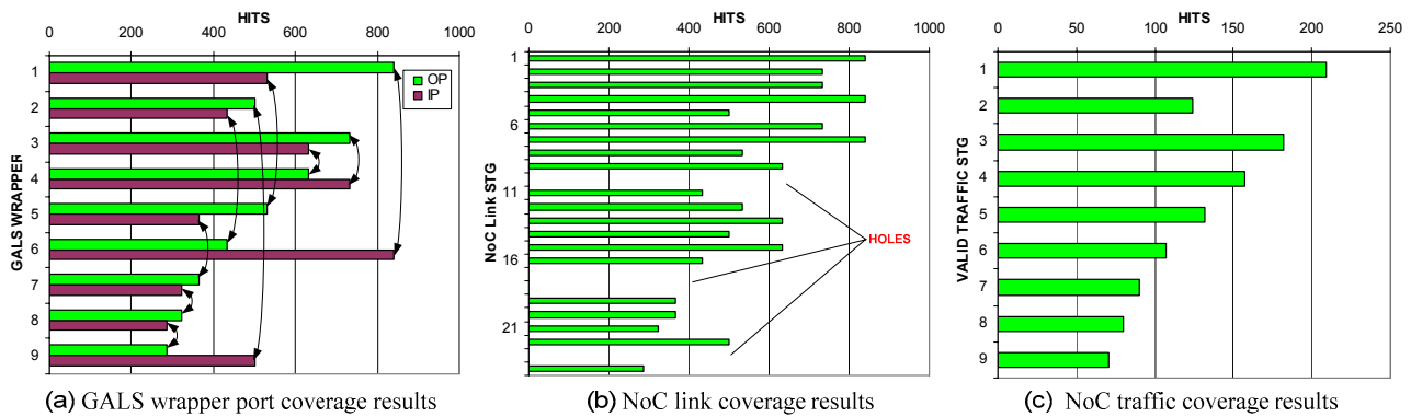
Figure 8: Verification example coverage results
