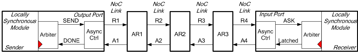
Figure 4: Verification Example: Module and NoC interfaces
