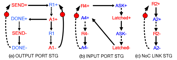
Figure 6: STG specifications
