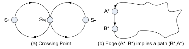
Figure 9: Proof of Lemma 1 and 3
