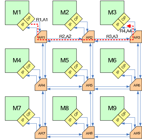
Figure 5: Design example. Multi-clock domain SoC with NoC
