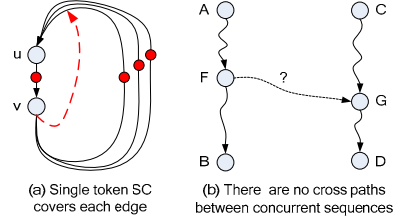
Figure 10: Proof of Lemma 5 and 7
