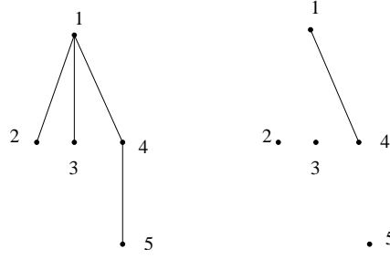
FIGURE 2. The graphs G_w (left) and G_w^1 (right) for the FK word w = 12131454
