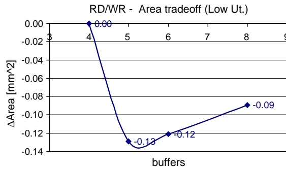
Fig. 8. \Delta Area—Optimization performed on RD/WR traffic (low utilization example).
