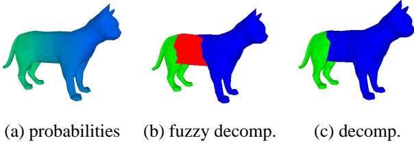
Figure 1. Algorithm [14] outline.
