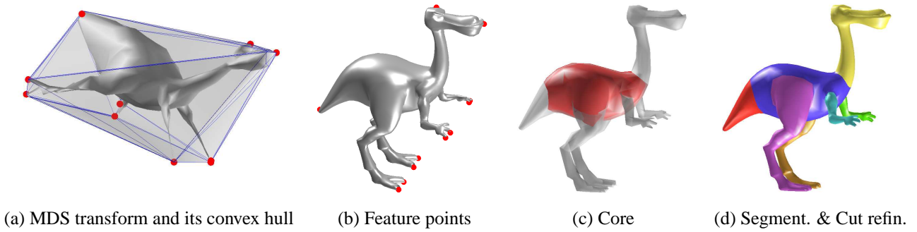
Figure 2. Algorithm [13] outline.
