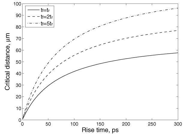
Fig. 6. Dependence of the critical line length d_{\text{crit}} on the rise time of the current load: I_{\text{max}} = 0.1 \text{ A} , V_{\text{dd}} = 1 \text{ V} , r = 0.007 \Omega/\mu\text{m} , and l = 0.5 \text{ pH}/\mu\text{m} . Note that d_{\text{crit}} is determined by t_r/t_f , increasing with larger t_f . The critical line length will shrink in future nanometer technologies as transition times become shorter.
