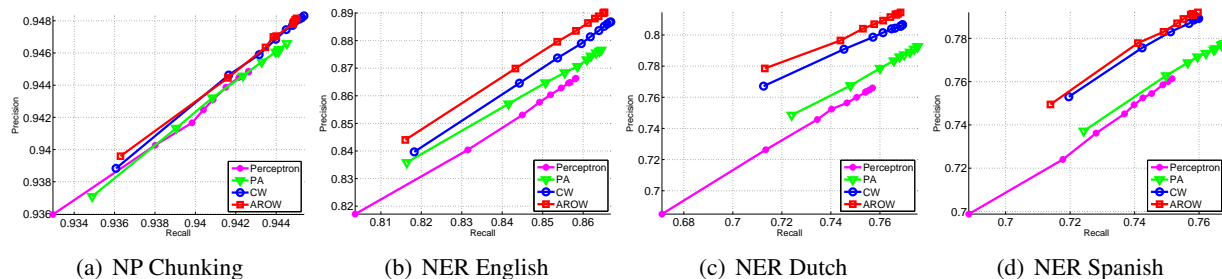
Figure 1: Precision and Recall on four datasets (four panels). Each connected set of ten points corresponds to the performance of a specific algorithm after each of the 10 iterations, increasing from bottom-left to top-right.
