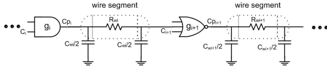
Figure 2. Cascaded logic gates with RC interconnect.
