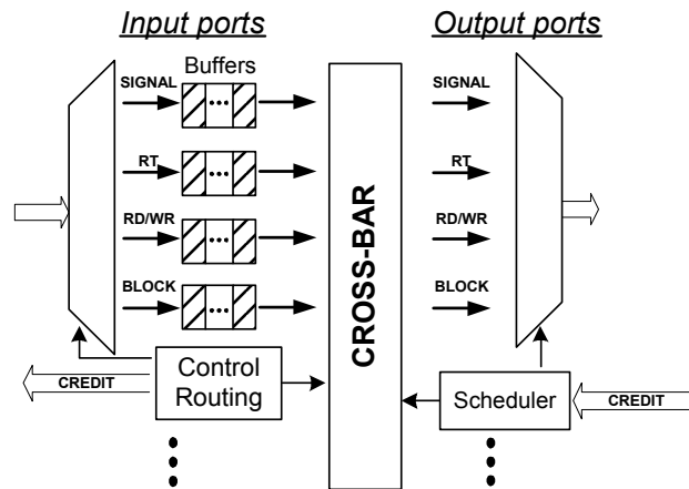
Figure 3. QNoC Router Architecture
