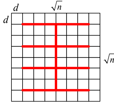
Figure 6. Non-Segmented Bus - interconnecting n communicating modules arranged in regular mesh, size of each is d \times d
