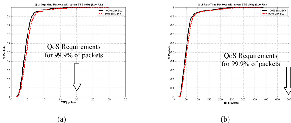
Figure 9. Degradation in ETE delay of Signaling (a) and Real-time (b) traffic when network bandwidth is dropped 10%. QoS requirements are still satisfied, in spite of this bandwidth reduction.
