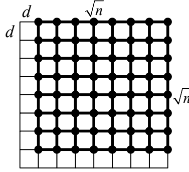
Figure 5. NoC – interconnecting n communicating modules arranged in regular mesh, size of each is d \times d
