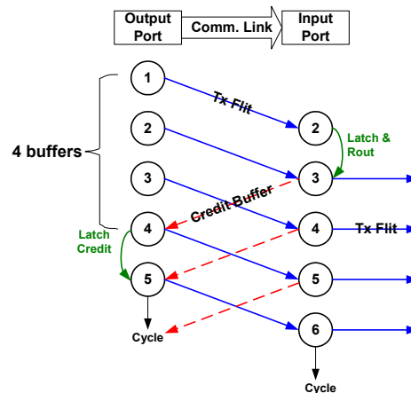
Figure 4. QNoC Transmission time-diagram demonstrating minimal buffering requirements preventing bubbles in a wormhole pipeline.
