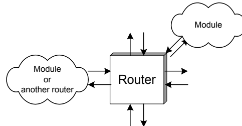
Figure 2. The router has up to five links and may connect to neighbor mesh routers or to chip modules.
