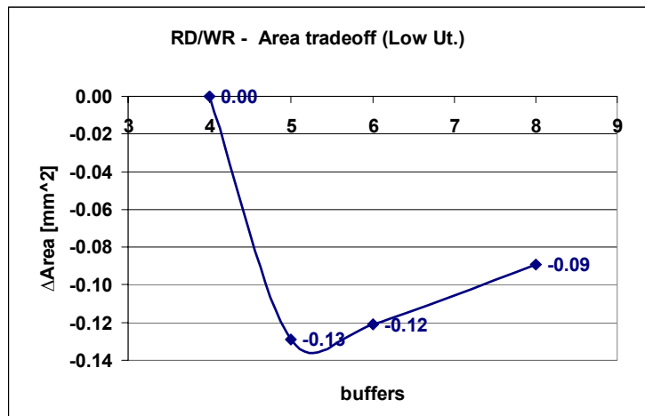
Figure 8. ΔArea – Optimization performed on RD/WR traffic (Low Utilization example)
