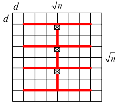
Figure 7. Bus segmented into \sqrt{n}/2 segments – interconnecting n communicating modules
