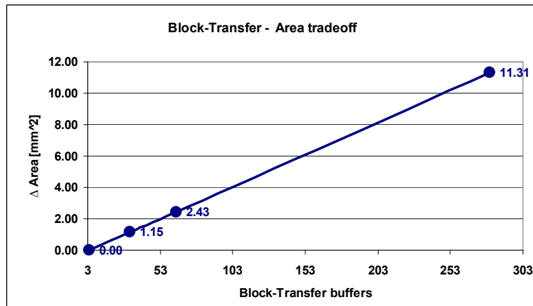
Figure 13. \Delta Area – Optimization performed on a Block-Transfer traffic – no cost minimization can be achieved
