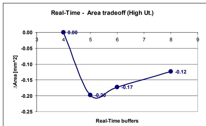
Figure 10. \Delta Area – Optimization performed on Real-Time traffic (High Utilization example)
