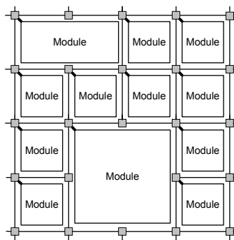
Figure 1. QNoC custom topology example - irregular mesh
