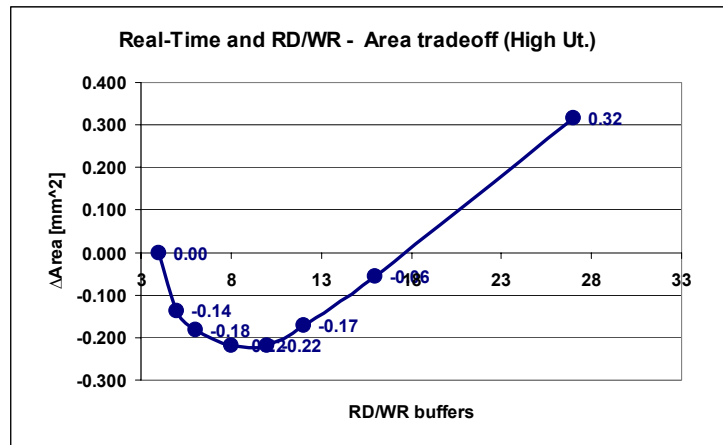
Figure 11. \Delta Area – Optimization performed on Real-Time and RD/WR traffic (High Utilization example)
