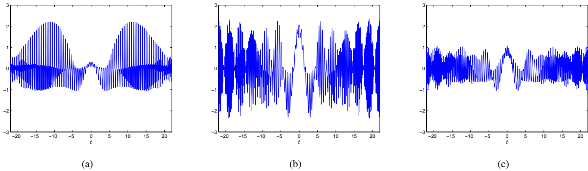
Fig. 6: Reconstructions of f(t) from its Gabor coefficients c_{k,l} . (a) Without processing c_{k,l} . (b) Consistent recovery, namely using d_{k,l} = (c * h_{\text{con}})_{k,l} as expansion coefficients. (c) Minimax-regret recovery, namely using d_{k,l} = (c * h_{\text{mx}})_{k,l} as expansion coefficients.
