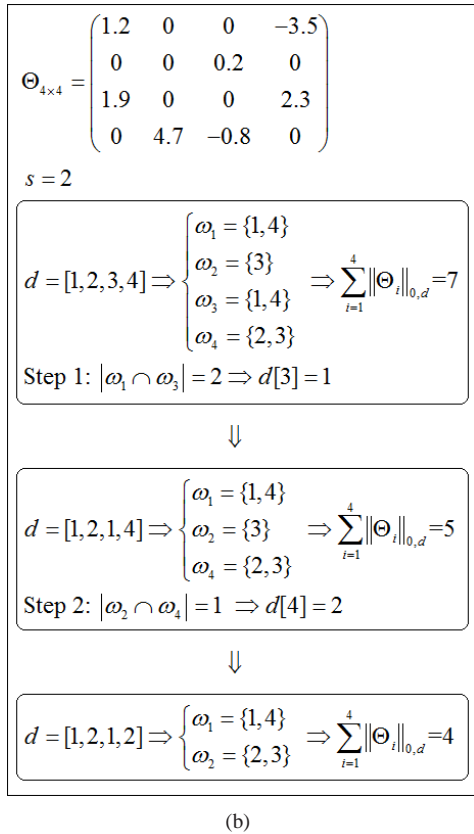
Fig. 2. (a) A flow chart describing the SAC algorithm. (b) A detailed example of the decision making process in the SAC algorithm.
