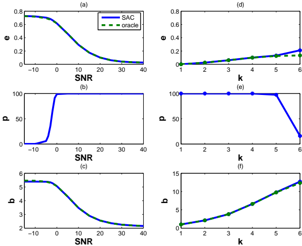
Fig. 3. Simulation results of the SAC algorithm. The graphs show e , p and b as a function of the SNR of the data signals for k = 2 (a, b, c), and as a function of k in a noiseless setting (d, e, f).
