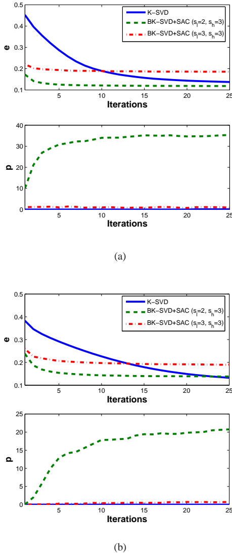
Fig. 6. Simulation results of our overall algorithm (BK-SVD+SAC) and the K-SVD algorithm, with maximal block size s_h = 3 . The graphs show the reconstruction error e and the recovery percentage p as a function of the number of iterations. (a) contains 12 blocks of size 2 and 12 block of size 3. (b) contains 30 blocks of size 2.
