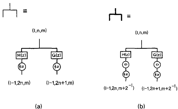
Fig. 6. A ‘parent’ node binary expansion according to SIWPD: (a) high- and low-pass filtering followed by a 2:1 downsampling, (b) high- and low-pass filtering followed by one sample delay ( D ) and subsequently by a 2:1 downsampling.
