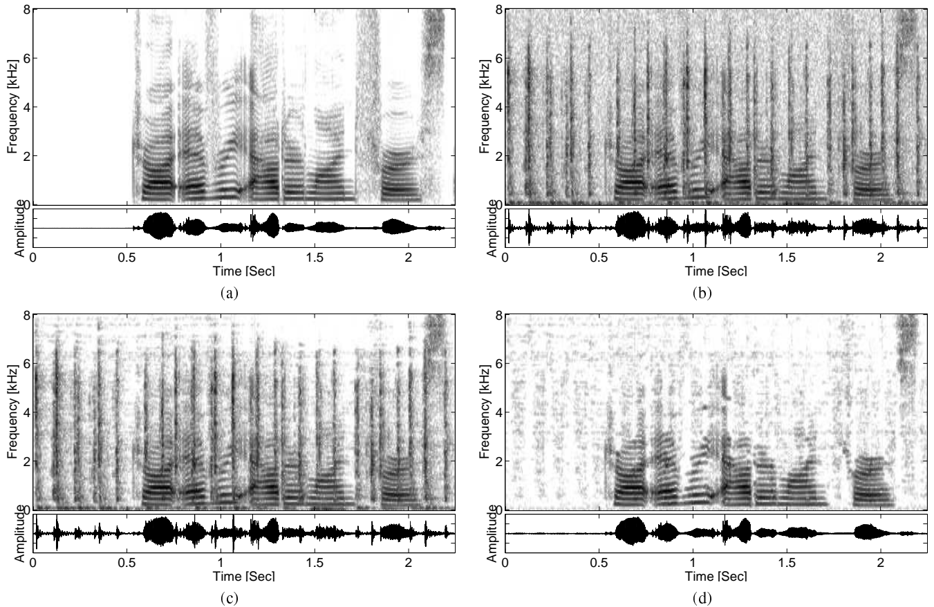
Fig. 2. Speech spectrograms and waveforms. (a) Clean signal (“Try any other line first”); (b) noisy signal (office noise including keyboard typing noise, SNR=0.8 dB); (c) speech enhanced by using the OM-LSA estimator; (d) speech enhanced by using the proposed algorithm.
